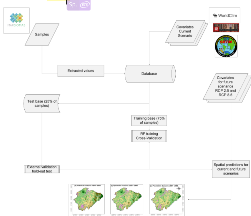
Figure 2. Overview of the main steps of methodological framework. RF = Random Forest; RCP = Representative Concentration Pathway.
