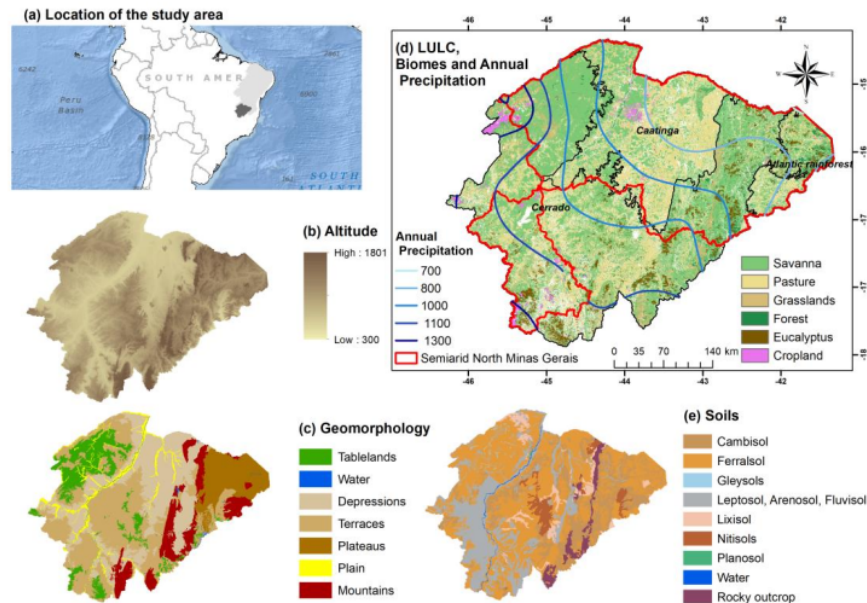
Figure 1. Characterization of the study area. (a) North of Minas Gerais State in the global context. (b) altitude; (c) geomorphology; (d) land use and cover (LULC) classes, biomes and mean annual precipitation distribution; and (e) soil types.
