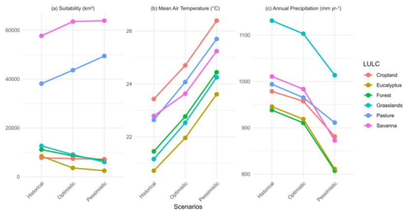
Figure 7. Quantitative comparison between changes in LULC and climate variables in the North of Minas Gerais. Suitability in km 2 of LULC classes (a); Mean air temperature for the extent of each LULC class (b); Annual precipitation for the extent of each LULC class (c). All variables are for the historical (1970 - 2000), optimistic, and pessimistic scenarios (2061 - 2080).
