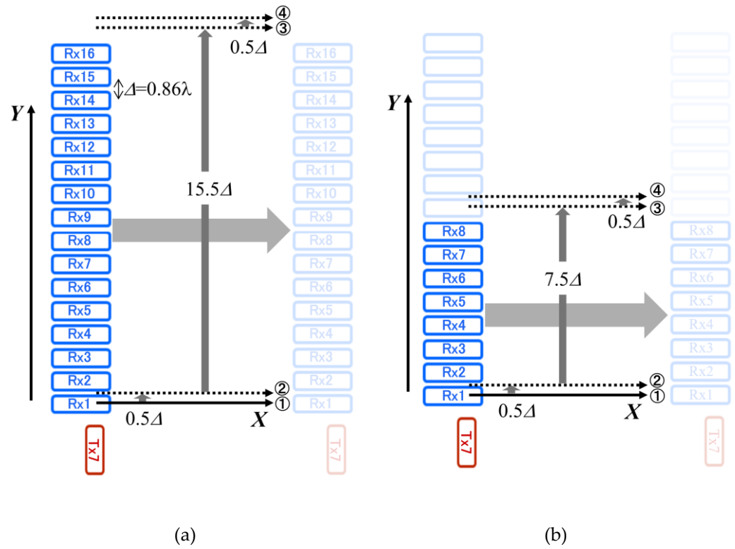
Figure 2. X-Y scanning method for antenna elements of the array. (a) Diagram of X-Y scanning using all Rx antennas from Rx1 to Rx16. (b) Diagram of X-Y scanning using eight Rx antennas from Rx1 to Rx8. Here, \Delta = 0.86\lambda is the distance between adjacent receive antennas.
