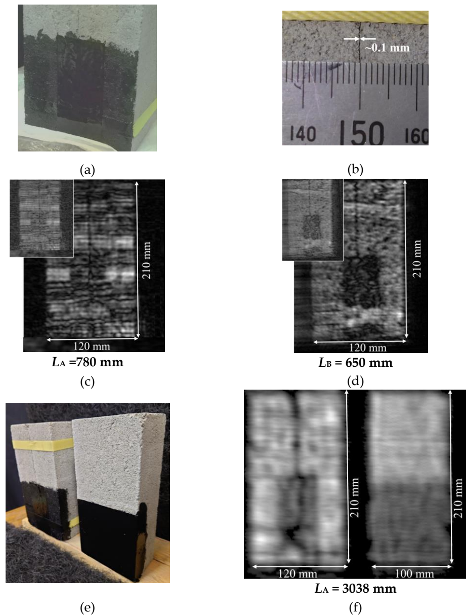
Figure 6. Comparison of MM-wave images of concrete blocks with GFR tape and black acrylic paint over the cracks. (a) Strongly bonded concrete blocks for observation. The contrast of the raw image is adjusted to show the position of the GFR tape under black acrylic paint. (b) Magnified view of the cracked area. It can be seen that the crack is about 0.1 mm wide. (c) MM-wave image observed at the target distance of L_A = 780 mm using system-A. (d) MM-wave image observed at the target distance of L_B = 650 mm using system-B. (e) Concrete blocks with (left) and without (right) cracks, thickly coated with acrylic paint over GFR tape. These were placed at a distance of L_A = 3038 mm from the radar module. (f) MM-wave images of concrete blocks with (left) or without (right) cracks.
