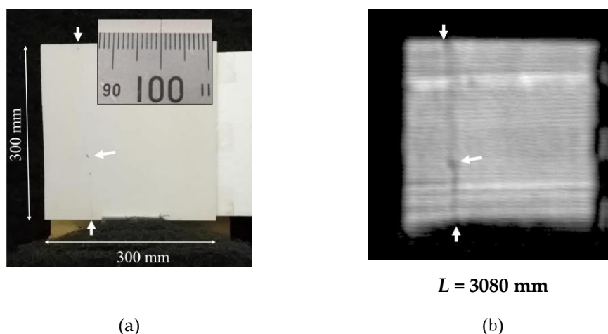
Figure 12. (a) A refractory board attached to a styrofoam board with double-sided tape. It was pre-split and set at L = 3080 mm. The insert shows the cracks of tens of \mu\text{m} width. The cracks cannot be seen from a distance. (b) MM-wave image of the refractory board at a distance of L = 3080 mm from the radar module. It can be seen that the crack streaks are imaged.
