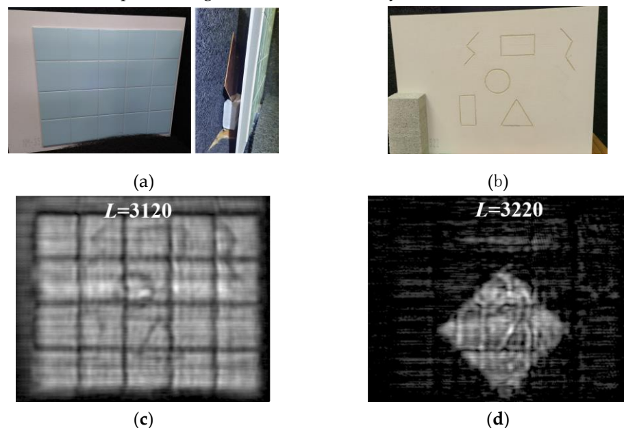
Figure 13. (a) Photograph of ceramic tiles and a refractory board attached with ceramic adhesives placed at L = 3115 mm and a copper plate placed at L = 3220 mm behind them for MM-wave transmission imaging. (b) Photograph of the pattern engraved on the surface of the refractory board bonded to the ceramic tile. (c) MM-wave image at the interface between ceramic tile and refractory
