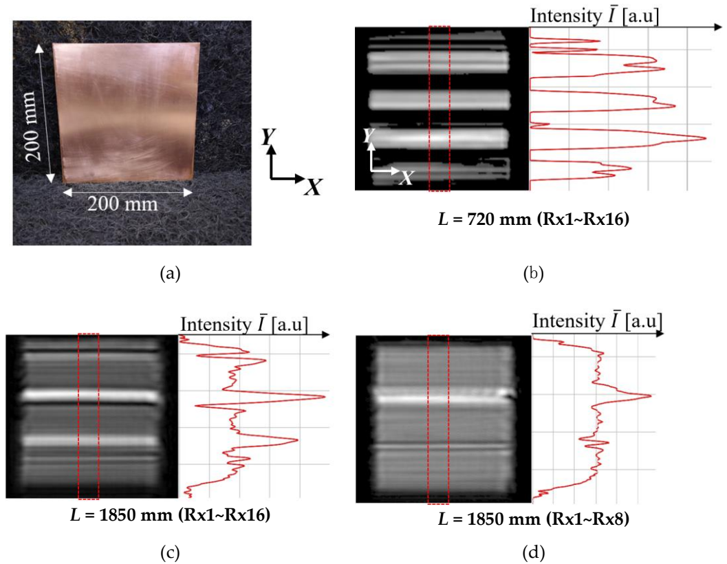
Figure 3. Influences of the distance L to the target and the number of receive antennas (Rx) used in the MM-wave image observations. (a) The 200 mm \times 200 mm flat copper plate for the measurements. (b) Condition of L = 720 mm with all receive antennas from Rx1 to Rx16. The left and the right figures show the observed MM-wave image and the distribution along the Y-axis of the averaged signal intensity \bar{I} within the red dotted rectangle inserted in the MM-wave image, respectively. (c) Result in the condition of L = 1850 mm with all receive antennas from Rx1 to Rx16. (d) Result in the condition of L = 1850 mm with 8 receive antennas from Rx1 to Rx8.
