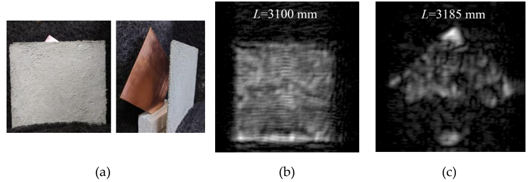
Figure 9. (a) Photographs of the thin concrete slab of 3.7 mm thickness placed at L = 3100 mm and the copper plate placed at L = 3185 mm behind it. (b) MM-wave image at position L = 3100 mm on the concrete surface and (c) MM-wave image at position L = 3185 mm on the copper plate surface.
