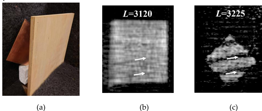
Figure 11. (a) A photograph of the composite plywood of 11.85 mm thickness placed at L = 3110 mm and the copper plate placed at L = 3225 mm behind it. (b) MM-wave image at position L = 3120 mm inside the composite plywood and (c) MM-wave image at position L = 3225 mm on the copper plate surface.
