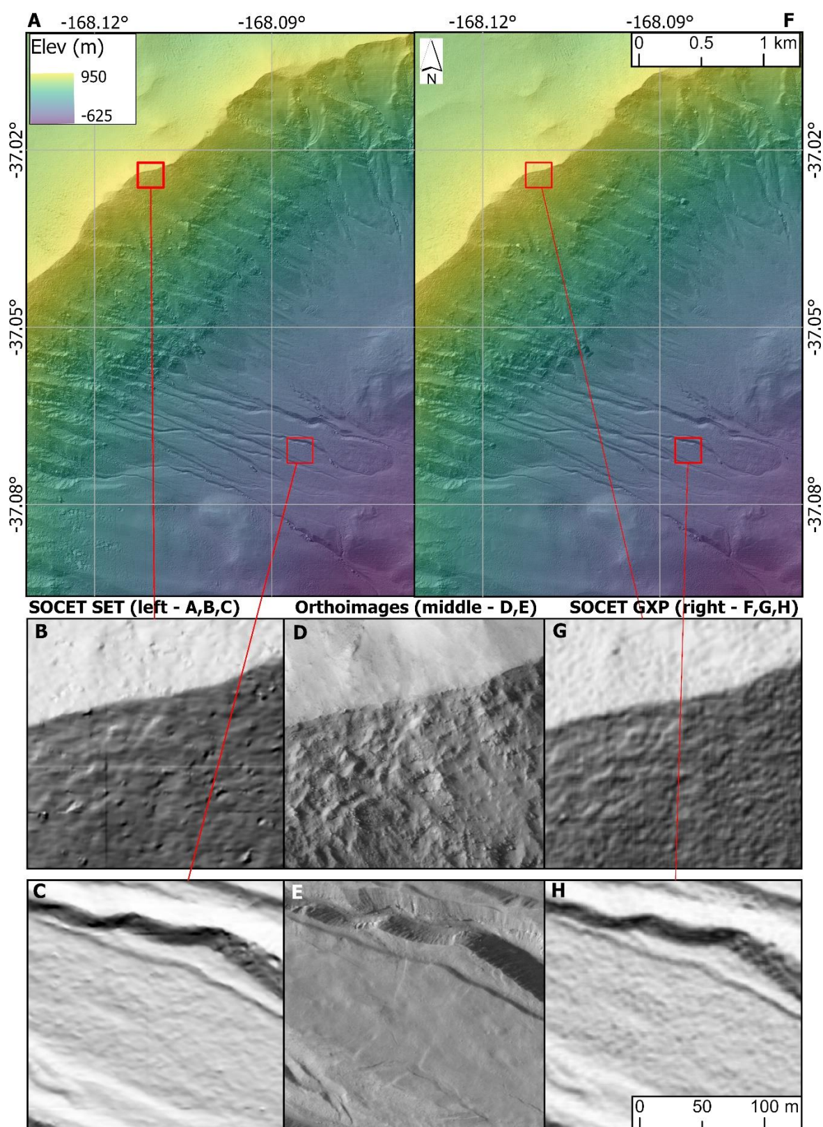
Figure 4. HiRISE DTM extract comparison as hillshades from SOCET SET (left, panels A–C) and SOCET GXP (right, panels F–H) of Triolet crater, Mars. Orthoimages from GXP are in panels D and E. See Section 3.2 for a detailed description.
