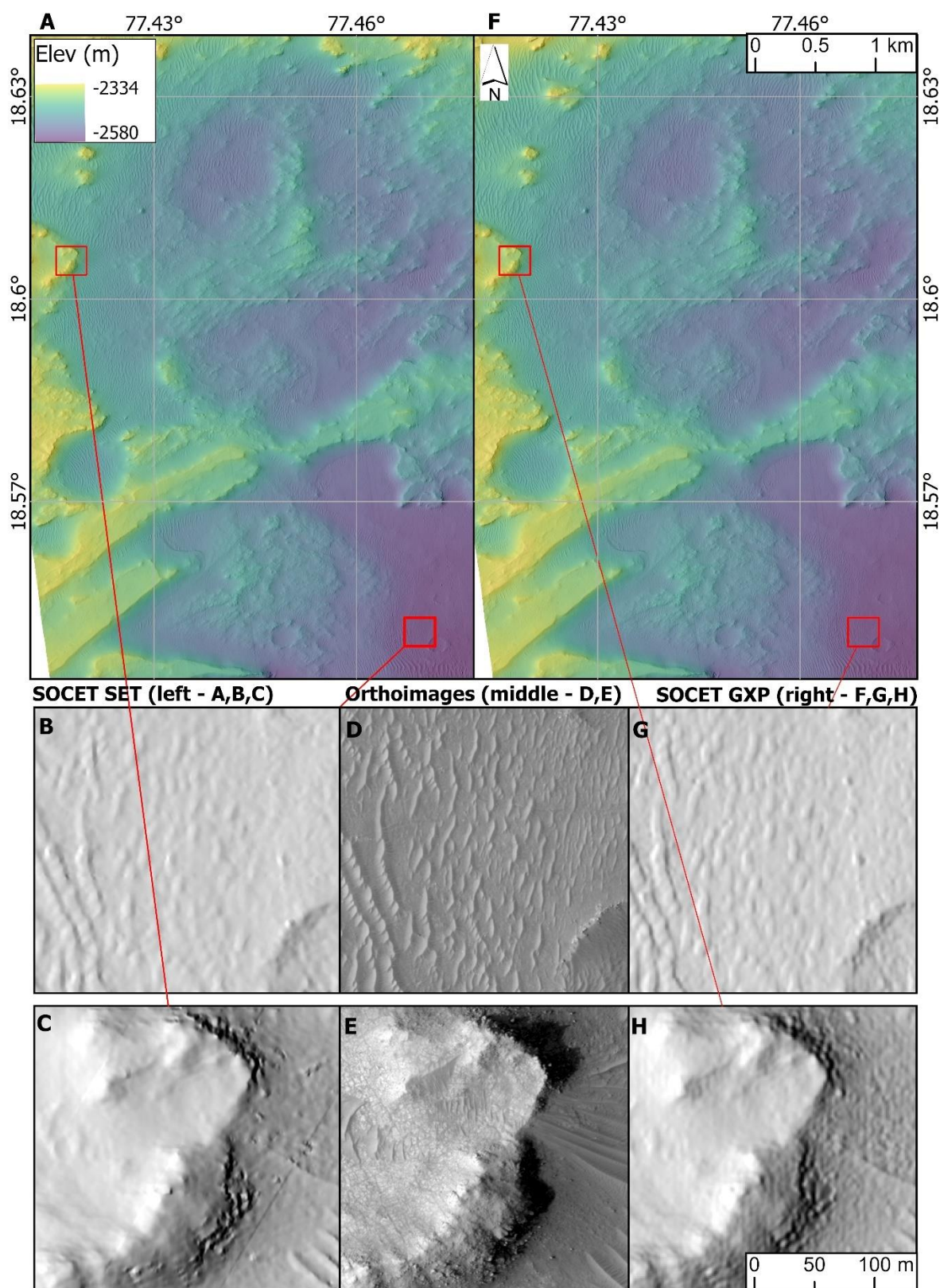
Figure 3. HiRISE DTM comparison visualized as hillshades of SOCET SET (left, panels A–C) and SOCET GXP (right, panels F–H) models from the same stereopair in Jezero crater, Mars. Orthoimages from GXP are in panels D and E. See Section 3.1 for a detailed description.
