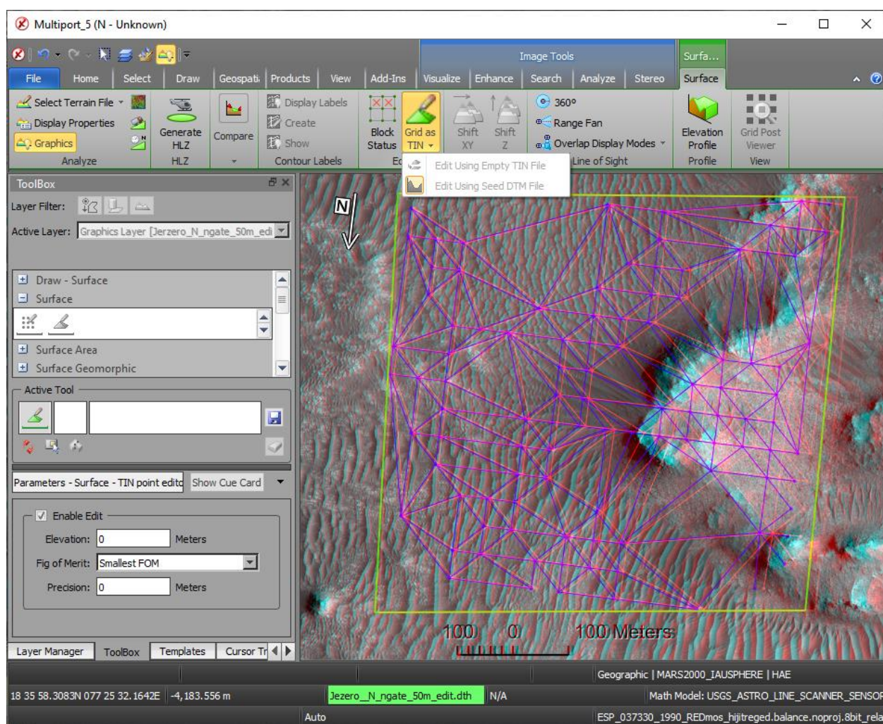
Figure 1. A screenshot of a multi-port viewer in SOCET GXP showing an anaglyph view for a HiRISE image stereo-pair within the floor of Jezero crater (77.69°E, 18.41°N). Using the newly added tool “Grid as TIN”, the user defines a small region as shown by the yellow box, where the original raster-based DTM was converted to a temporary triangular irregular network (TIN) for vertex editing. Once the user completes their updates to the TIN, the tool will then convert the allocated region back to a raster-based pixel grid for further pixel-based editing.
