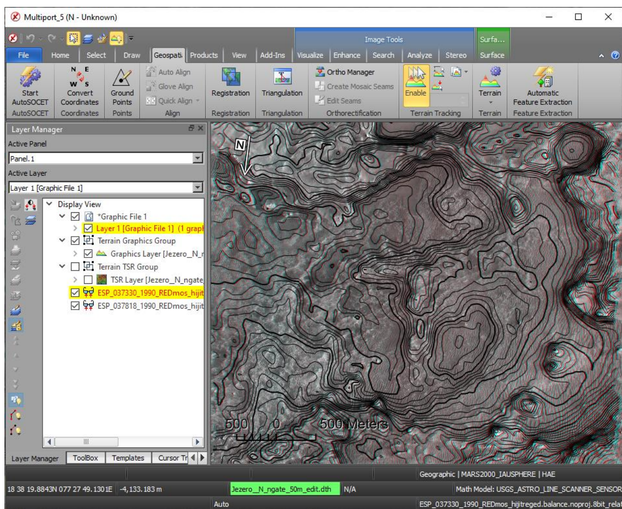
Figure 2. A screenshot of a SOCET GXP Multiport showing an anaglyph view for a HiRISE image stereo-pair (ESP_037330_1990, ESP_037818_1990, red channels) within the floor of Jezero crater (77.69°E, 18.41°N). 4-meter interval contours are shown to highlight a visual representation for the stereo-derived DTM. While editing can be performed in this anaglyph mode, most workstations, specifically configured for DTM editing, will have a high-end Graphics Processing Unit (GPU) driving two Liquid Crystal Displays (LCDs) mounted on a specially designed stand. A passive polarized mirror bisects the two monitors allowing the user, who is wearing polarized eyeglasses, to view the left and right monitors separately. The SOCET GXP application, using the available rigorous camera model, provides dynamic adjustments to the left and right images, resulting in the perception of depth. This is how a user can visually verify the quality of the DTMs point-by-point and manually edit any mismatched points (also called blunders).
