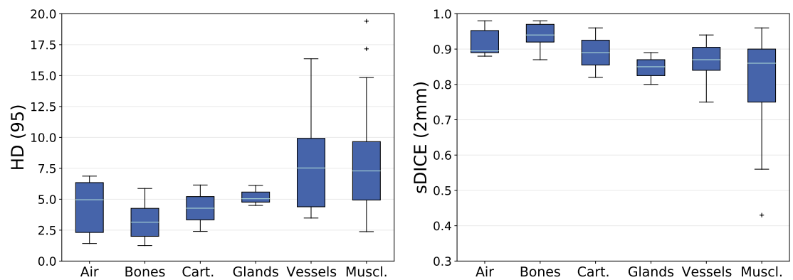
Figure 4. Mean HD and mean sDICE values between manual delineation and predicted label for each anatomical structure grouped by their tissue types. Means are calculated over all test patients for that the structure is present (maximum 18 test patients). Box plots show the median (cyan) and outliers (cross). Box (blue) reaching from the first quartile (Q1) to the third quartile (Q3), whiskers reaching to the 1.5 interquartile range. Quantities per group were: Air (6), Bones (11), Cartilages (2), Glands (3), Muscles (26), and Vessels (11).
