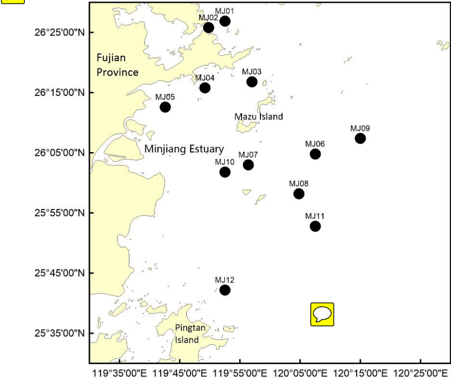
Figure 1. Bottom trawl sampling sites in the Minjiang Estuary and its adjacent waters.
