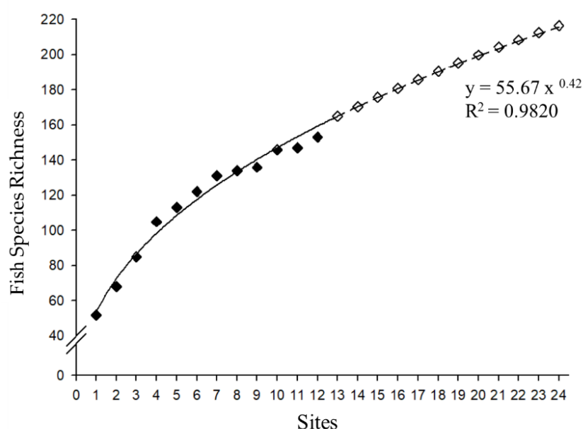
Figure 5. The accumulation curve of fish species richness with the number of stations in the Minjiang Estuary.
