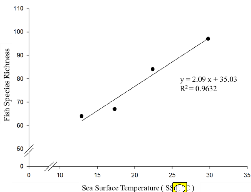
Figure 3. The relationship between fish species richness and SS the Minjiang Estuary and its adjacent waters.
