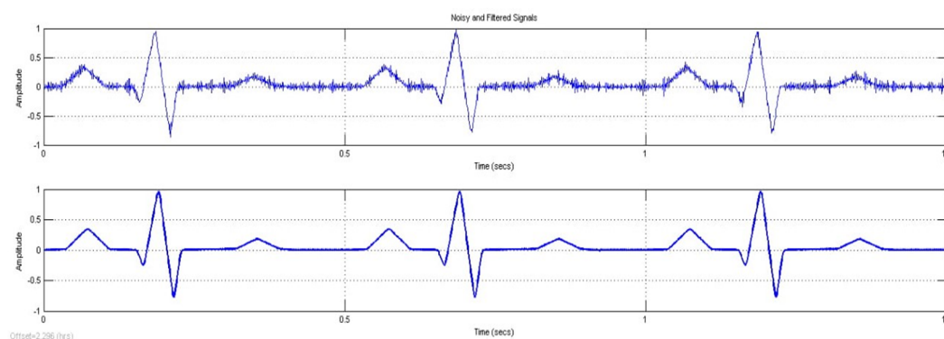
Figure 11. ECG recording with and without noise (Source: Bellos, Papadopoulos [30])
