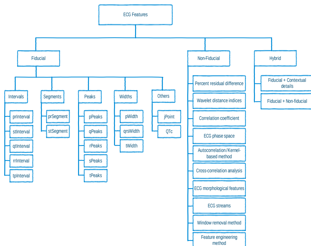
Figure 12. Taxonomy of features for ECG interpretation and diagnosis
