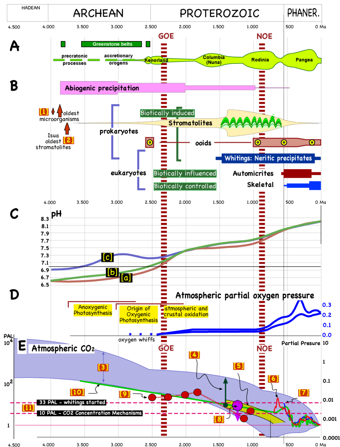
Figure 2. Carbonate precipitation nodes, genetic macroevolution rates, and estimates of oxygen and CO 2 in the atmosphere. A: Supercontinents and crustal growth; precratonic, accretionary orogens and supercontinents assembly (redrawn from [11]). B: carbonate precipitation modes through Earth's history (multiple sources). [1]: Oldest fossils [11]. [2]: Isua oldest stromatolites [13]. C: pH evolution from [14]; a: nominal model, in which the median Archean surface temperature is slightly higher than modern surface temperatures. Archean land fraction was anywhere between 10% and 75% of modern land fraction; b: no Archean land endmember scenario; c: model with assumed 100 ppm Proterozoic methane and 1% Archean methane levels. D: Maximum and minimum estimates of atmospheric partial oxygen pressure (after [15]). E: estimates of atmospheric CO 2 concentration; [3] from [16], upper and lower boundaries reflect average surface temperature for an ice-free (20°C) and ice covered (5°) Earth; [4] Acritarch isotopic composition [17]; [5] C-isotope reservoir modeling
