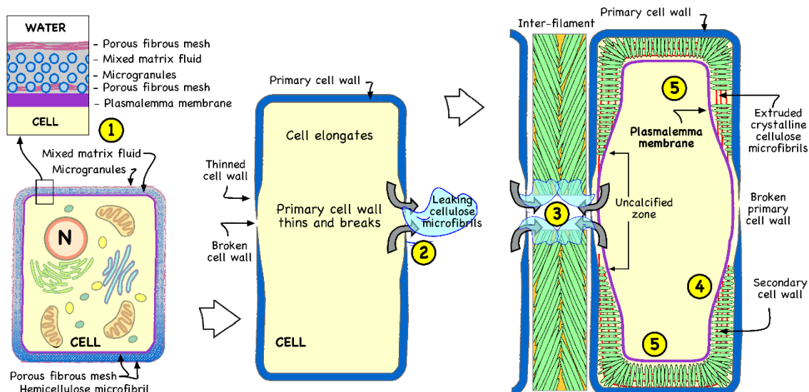
Figure 11. Skeleton formation in red algae (based on Nash et al. [74]). (A) Primary cell wall is forming. Hemicellulose microfibrils act as nucleating substrate for micro-granules. (B) Cellulose microfibrils extrude from plasma membrane and leaks through broken primary cell wall. (C) Inter-filament grains initiate attached to the external part of the primary cell wall and growth in the leaked cellulose microfibril. (D) Secondary cell wall thickens, extruded cellulose microfibrils stops leaking and mineralizes as Mg-calcite. (E) Plasmalemma pushed inwards as cellulose microfibril continues to extrude and mineralize. Secondary cell wall fully formed.
