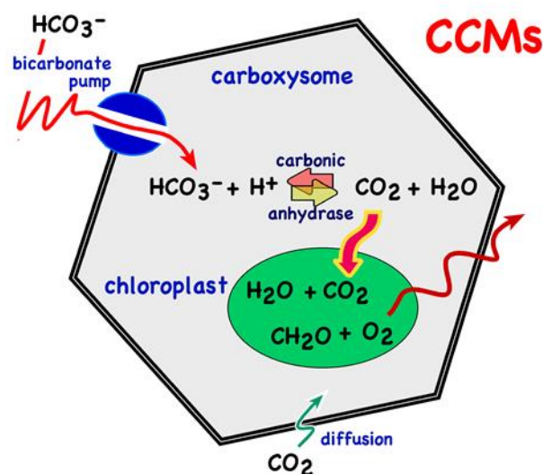
Figure 4. Central to the cyanobacterial CCM is the carboxysome, a cellular micro-compartment containing the RuBisCo and a carbonic anhydrase (CA) that by converting \text{HCO}_3^- into \text{CO}_2 rises \text{CO}_2 concentration up to 1000-fold around the active site of RuBisCO [40].
