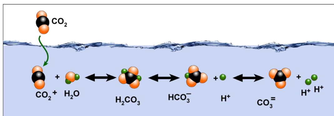
Figure 3. In an aqueous solution, carbonate, bicarbonate, carbon dioxide, and carbonic acid exist together in a dynamic equilibrium. When \text{CO}_2 is absorbed by seawater, a series of chemical reactions increase the concentration of \text{H}^+ and cause the seawater acidity to increase. When calcium carbonate (e.g., limestone) reacts with acidic free hydrogen ( \text{H}^+ ) ions in seawater, the solid calcium carbonate dissolves, releasing free calcium ( \text{Ca}^{2+} ) ions and free bicarbonate ( \text{HCO}_3^- ) ions.
