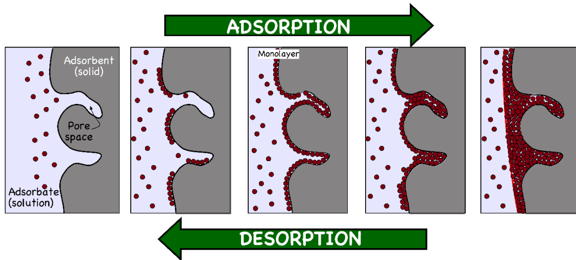
Figure 6. Simplified diagram of the adsorption process. Atoms, molecules or ions adhere to a surface by weak residual forces (e.g., van der Waals, electrostatic). It can be multilayer or monolayer.
