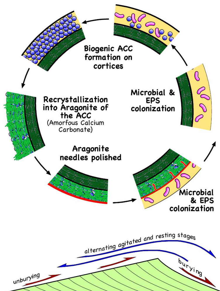
Figure 9. Conceptual multiphase model for the oolite cortex accretion, based on [64,65].
