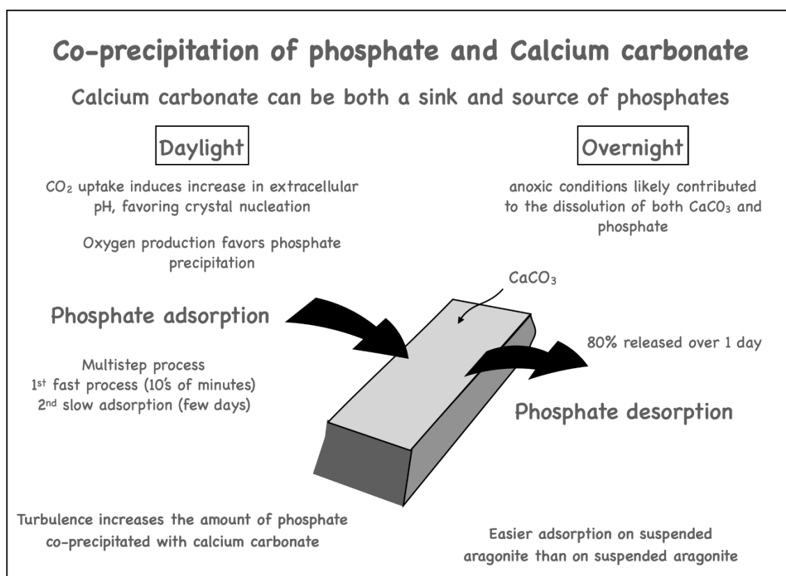
Figure 7. Co-precipitation of phosphate and calcium carbonate.
