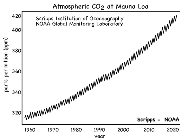
Figure 1. CO 2 concentrations in the atmosphere, started by C. David Keeling of the Scripps Institution of Oceanography in March 1958.
