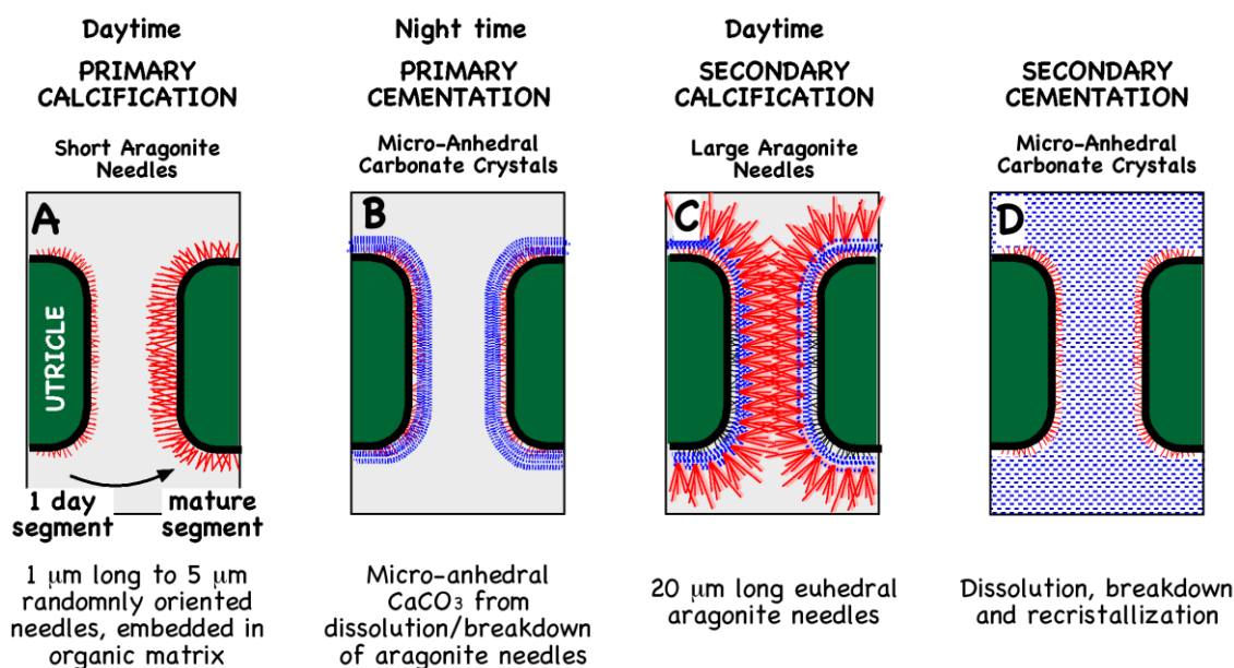
Figure 10. Calcification stages of Halimeda [72,73]. A: Growth of short skeletal needles on the utricle wall; B: Recrystallization of short needles to micron-sized anhedral crystals. C: secondary calcification by long and dense euhedral skeletal aragonite needles, D: the primary inter-utricular space In the rim of the segment is filled with micron-sized anhedral crystals.
