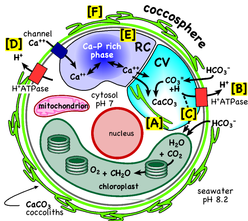
Figure 12. Calcification processes in coccolithophorids (based on [82, 83, 84, 85]. [A] Coccolith formation occurs within the Golgi-derived coccolith vacuole (CV). Intracellular \text{CaCO}_3 precipitation from bicarbonate ( \text{HCO}_3^- ) releases equimolar \text{H}^+ that must be rapidly removed from the CV to maintain pH for \text{CaCO}_3 precipitation [B]. Some \text{H}^+ may be utilized by photosynthesis [C]. Not yet fully understood, it is hypothesized \text{Ca}^{2+} to be recruited through Ca-channels and V-type ATPase pumps [D]. A reservoir compartment (RC) concentrates \text{Ca}^{2+} and \text{P}_i [E]. The coccolith-associated polysaccharide [F] may drive the \text{Ca}^{2+} from the coccosphere into the RC, from where only \text{Ca}^{2+} is derived to the coccolith vesicle (CV) and phosphorous is diverted to the cell for algal growth and reproduction. Transfer of \text{Ca}^{2+} from the RC into the CV uses \text{Ca}^{2+} channels and transporters.
