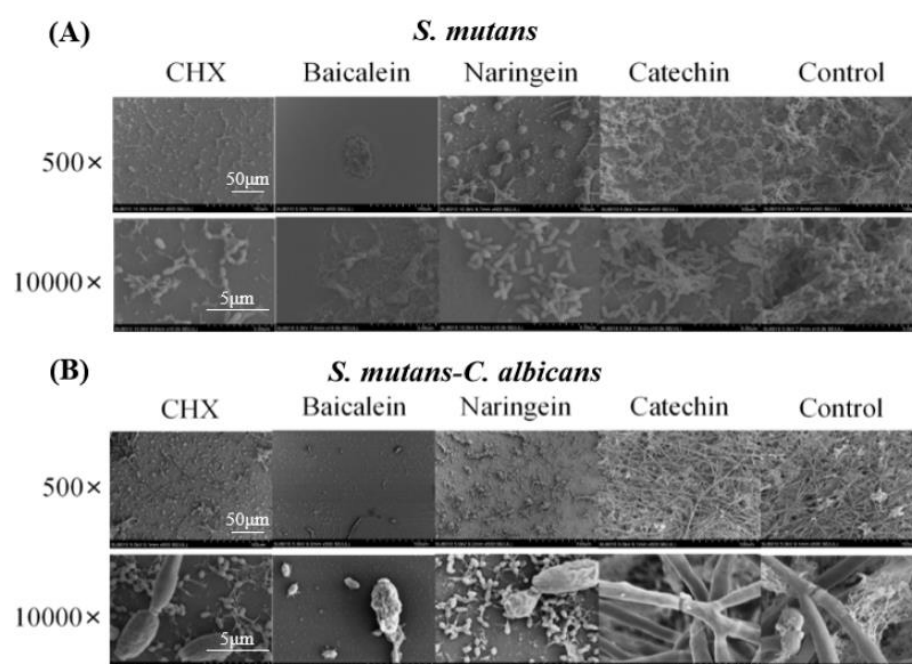
Figure 2. SEM observation of (A) S. mutans , and (B) S. mutans-C. albicans biofilms after flavonoids or CHX treatment.
