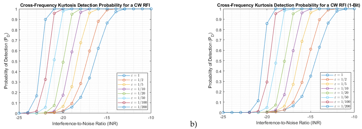
Figure 5. Probability of detection (PD) as a function of the INR, parameterized as a function of the variance reduction factor ( \epsilon ), for (a) multi-bit, and (b) 1-bit quantization.
