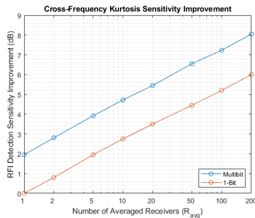
Figure 6. Sensitivity improvement of the RFI detection [dB] as a function of the number of receivers averaged ( R_{avg} ) for the multi-bit and 1-bit quantization approaches.
