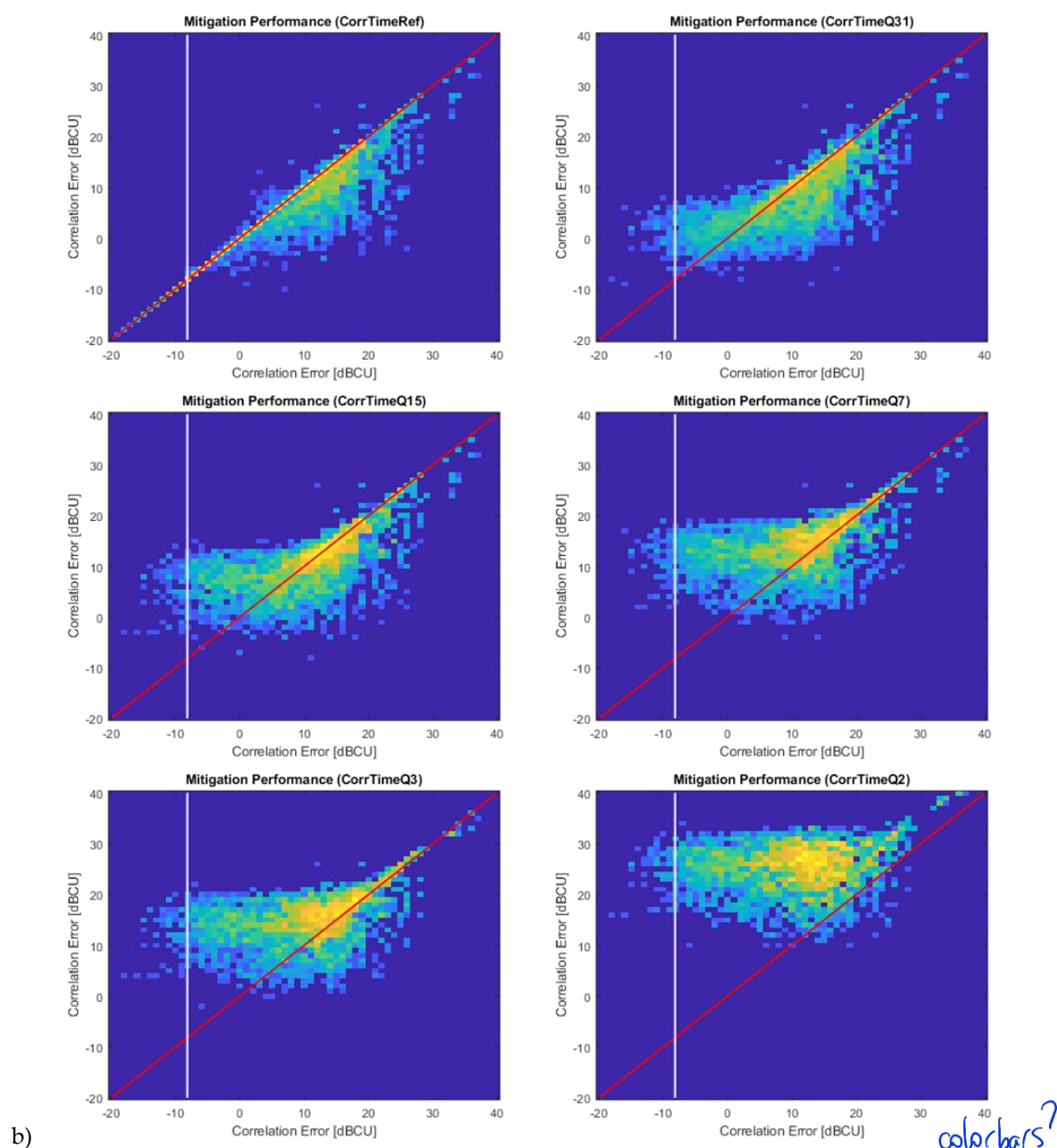
Figure 8. Mitigation performance in the a) frequency-, and b) time-domains as a function of the quantization levels: 2, 3, 7, 15, and 31 and multi-bit reference case (top left).
