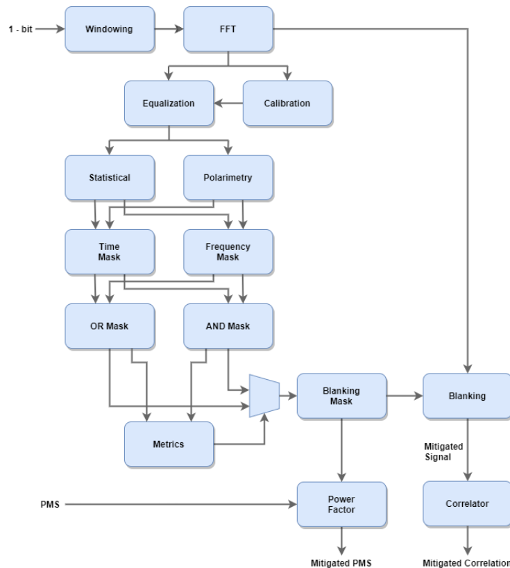
Figure 1. Overall block diagram of the RFI mitigation proposed algorithm.
