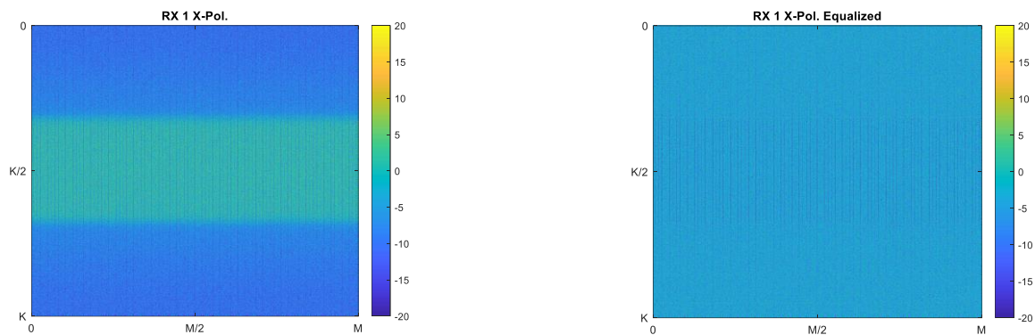
Figure 2. Modulus square of the STFT of the X-pol. at a sample receiver (a) before, and (b) after equalization. The vertical lines appearing in both figures are due to the clipping of the input receiver signal due to the strong RFI signal.
