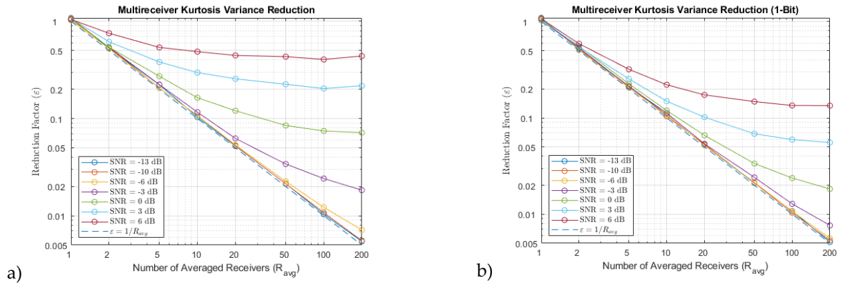
Figure 4. Multi-receiver Kurtosis variance reduction as a function of the number of receivers averaged ( R_{avg} ) and SNR for a) multi-bit, and b) 1-bit quantization. SNR is the power relation between correlated divided by uncorrelated noise power.
