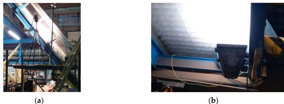
Figure 3. (a) Image collection apparatus for L/L_t = 0.49 (which is equivalent to that on L/L_t = 0.88 ) using frontal illumination. (b) Image collection apparatus for L/L_t ranging from 0.88 to 0.89 using back illumination.
