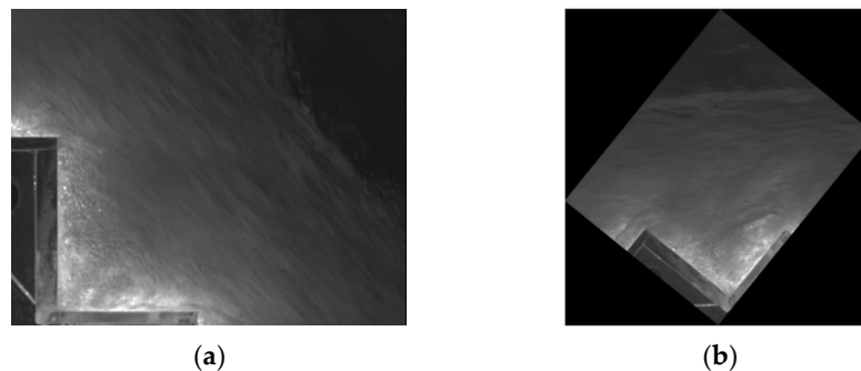
Figure 5. Image corresponding to L/L_t = 0.49 and d_c/h = 2.38 : (a) Original frame; (b) Rotated frame 51.3° counterclockwise.
