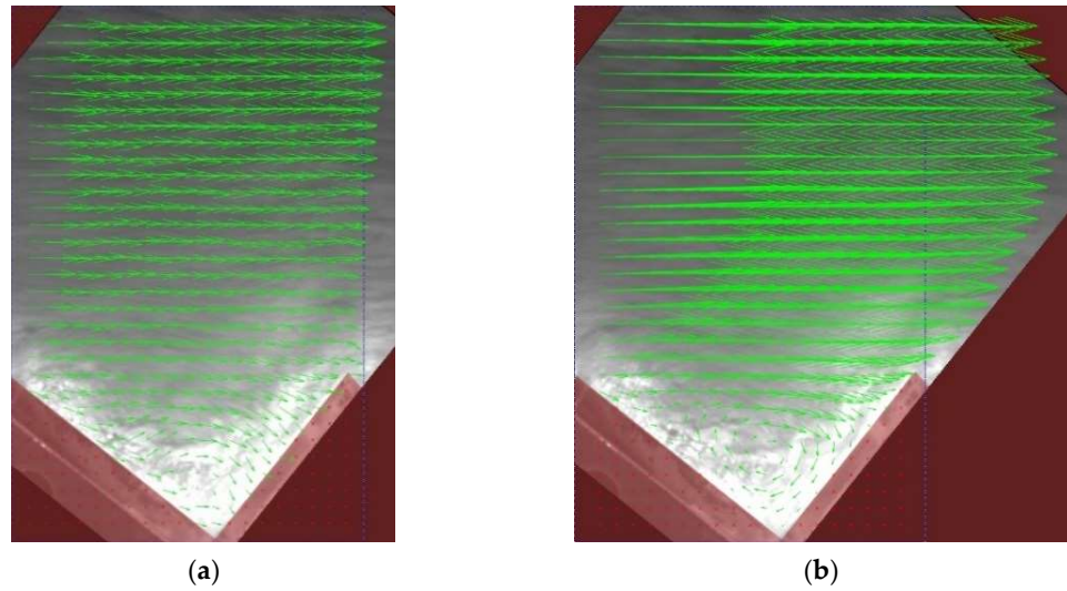
Figure 10. Average velocity field obtained at L/L_t = 0.49 for d_c/h = 2.38 and (a) 200 fps (b) 400 fps, when reducing the interrogation area in 3 steps from 288 to 144, then to 72, and then to 36 pixels.
