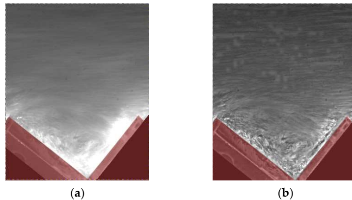
Figure 7. Frame 1104 corresponding to d_c/h = 2.38 and 200 fps. (a) Original image. (b) Image after a CLAHE filter and contrast improvement (minimum 0 and maximum 0.95).
