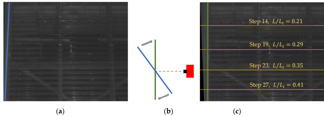
Figure 4. (a) Original frame #0001 of video 0 (without water, 200 fps); the blue line is the foot of the right sidewall of the chute. (b) Image folding (profile view). (c) Folded original frame #0001 of video 0; the green line represents the foot of the folded right sidewall of the chute.
