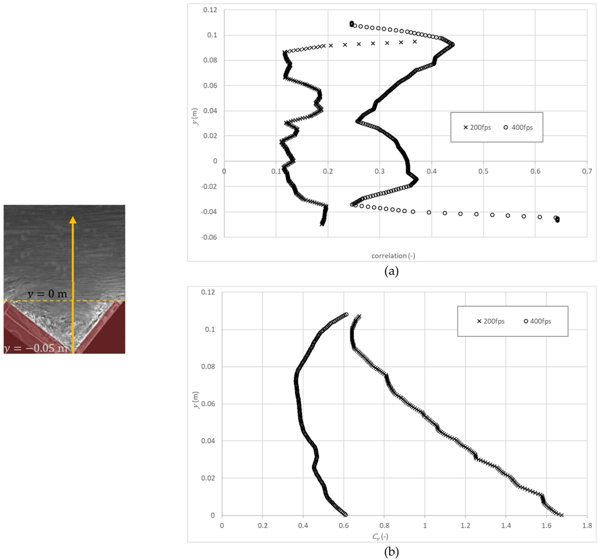
Figure 12. Time-averaged correlation between consecutive frames (a) and coefficient of variation (b) obtained at L/L_t = 0.49 for 200 fps and 400 fps. The scheme includes the layout of the vertical where the velocities were obtained. The dashed line represents the pseudo-bottom ( y = 0 ).
