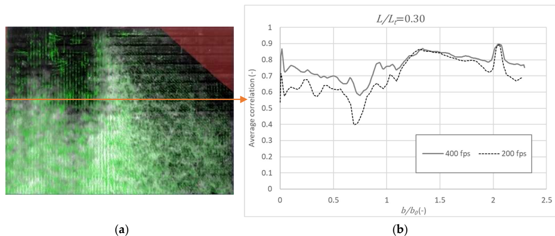
Figure 8. (a) Gross frontal velocity field obtained in frame 691 for d_c/h = 2.38 for an interrogation area with 4 steps using decreasing size of the interrogation areas from 300 px to 50 px. (b) Time-averaged correlation for 400 fps and 200 fps across the chute width at L/L_t = 0.30 .
