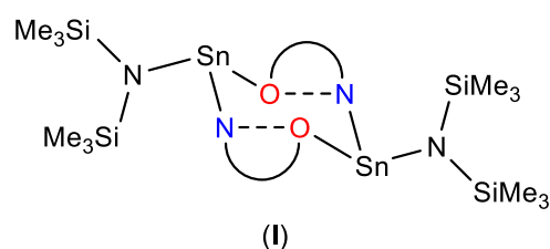
Scheme 4. Schematic showing the coordination of the {hp} ligand in complex 1 .
