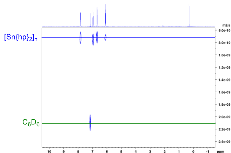
Figure 2. Plot showing the ^1\text{H} DOSY NMR spectrum for compound 2 (298K).
