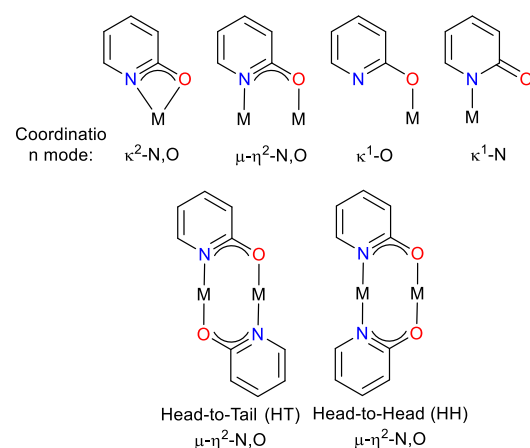
Figure 2. Overview of the N,O donor pro-ligands, hpH, hqH and hbqH used in this study (A), and the common coordination modes observed for the 2-hydroxypyridinato (hp) ligand (B).
