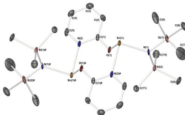
Figure 4. The molecular structure of one of the two full molecules of complex 1 present in the unit cell. Symmetry transformations used to generate equivalent atoms: #1 -X, -Y, 1-Z . Thermal ellipsoids are shown at 50% probability. Hydrogen atoms have been omitted for clarity.
