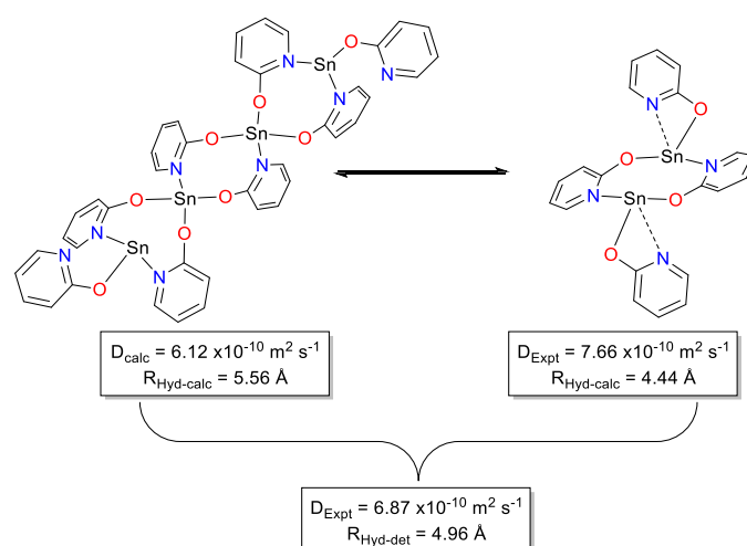
Scheme 2. Proposed Tetramer Dimer equilibria observed for 2 .
