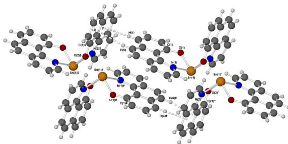
Figure 7. A representation of the H-Bonding and \pi - \pi stacking observed in the solid-state structure of 5 . Bond lengths: H(4)-(1) cent = 2.658(12)\text{\AA} and H(6)-(2) cent = 3.227(12)\text{\AA} . Inter-
