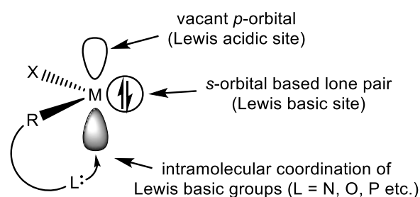
Figure 1. Stabilization of stannylene [\text{Sn}(\text{R-L})_{2-x}(\text{X})_x] complexes.
