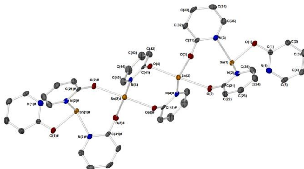
Figure 5. The molecular structure of complex 2 . Symmetry transformations used to generate equivalent atoms: #1 3/2-X, Y, 1-Z. Thermal ellipsoids are shown at 50% probability. Hydrogen atoms have been omitted for clarity.
