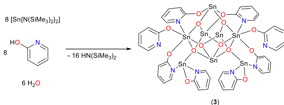
Scheme 6. Formation of the Sn(II) oxo cluster, [\text{Sn}_6(\mu_3\text{-O})_6(\text{OR})_4:\{\text{Sn}^{\text{II}}(\text{OR})_2\}_2] ( 3 ) ( \text{R} = \text{C}_5\text{H}_4\text{N} ).
