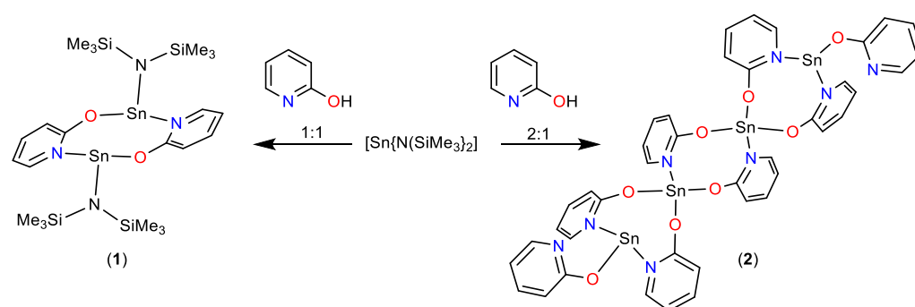
Scheme 1. Formation of complexes 1 and 2 .
