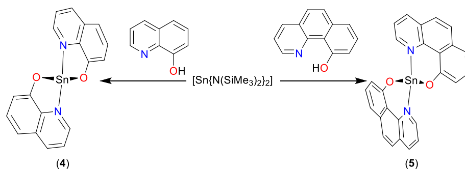
Scheme 3. The synthesis of complexes 4 and 5 .
