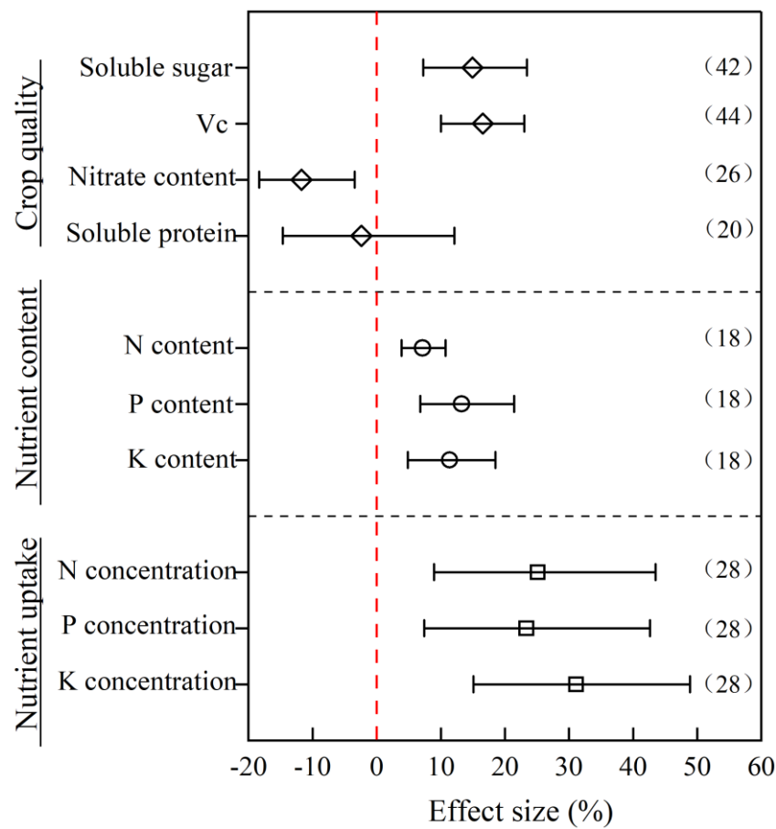
Figure 4. Effect size analysis of various factors on crop quality and nutrient uptake under negative pressure irrigation compared with conventional irrigation conditions .
