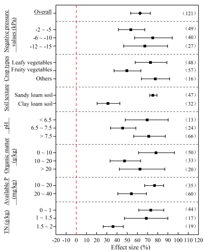
Figure 3. Effect size analysis of various factors on water use efficiencies under negative pressure irrigation compared with conventional irrigation conditions.
