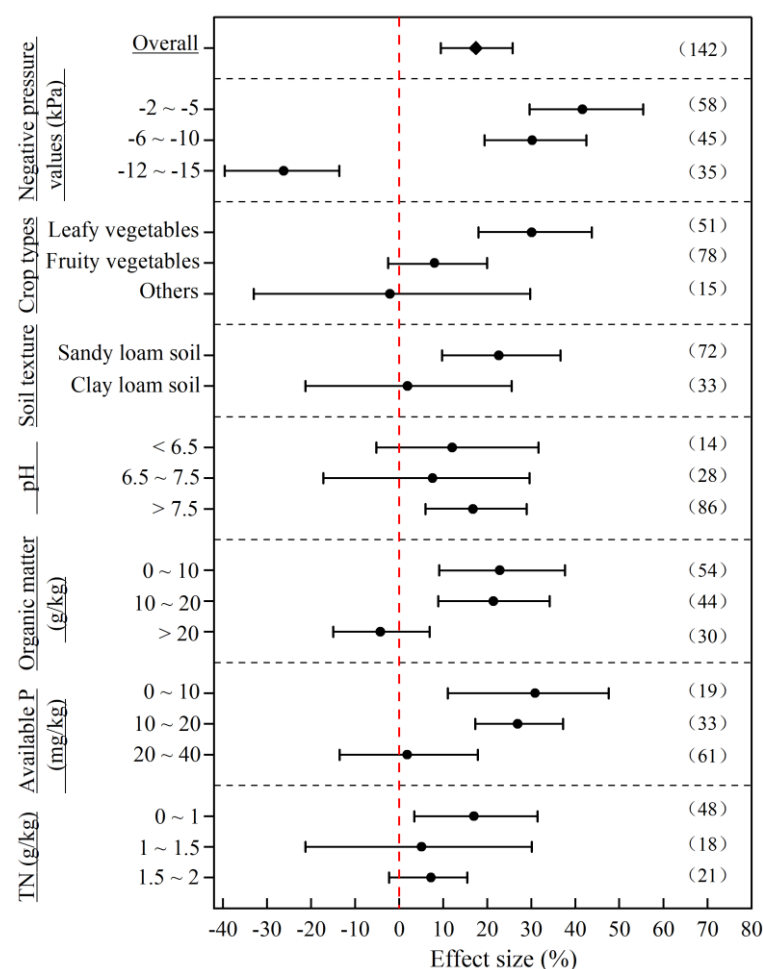
Figure 2. Effect size analysis of various factors on crop yields under negative pressure irrigation compared with conventional irrigation conditions.
