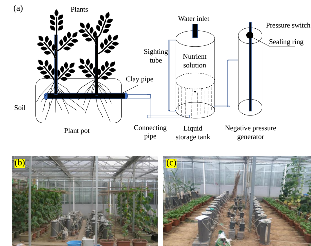
Figure 1. Schematic of plant growth when using a negative pressure irrigation system (a). Negative pressure irrigation applied to cucumber (b) and rapeseed (c) in greenhouse production.
