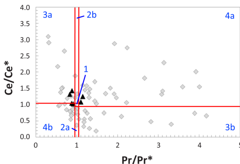
Figure 6. (\text{Ce}/\text{Ce}^*)_{\text{N}} vs. (\text{Pr}/\text{Pr}^*)_{\text{N}} plot (after [80]) of five-point averages along the transect across the cortex of MOR 2598 recorded by LA-ICPMS. Separate fields (labeled by blue text) are as follows: 1, neither Ce nor La anomaly; 2a, no Ce and positive La anomaly; 2b, no Ce and negative La anomaly; 3a, positive Ce and negative La anomaly; 3b, negative Ce and positive La anomaly; 4a, negative Ce and negative La anomaly; 4b, positive Ce and positive La anomaly. Measurements from the outer 1 mm of the external cortex are plotted as black triangles, and all measurements from deeper within the bone are plotted as grey diamonds. (\text{Ce}/\text{Ce}^*)_{\text{N}} vs. (\text{Pr}/\text{Pr}^*)_{\text{N}} anomalies calculated as in the Materials and Methods section of the text.
