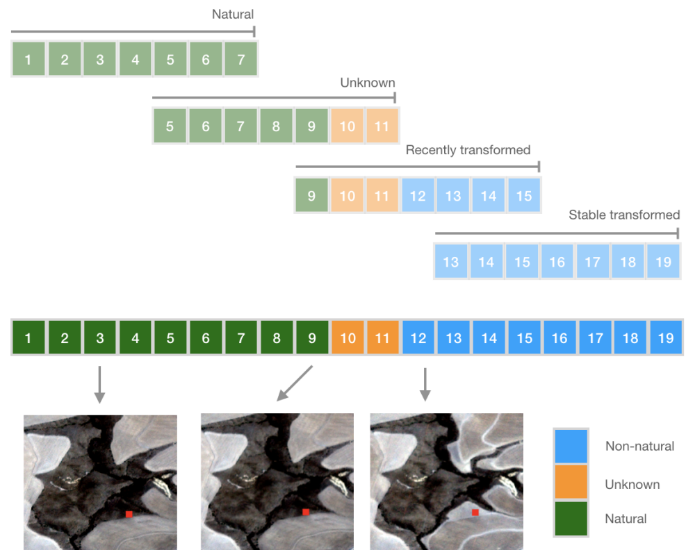
Figure 2. The approach used for labelling time series to enable continuous classification of change. Each step in the sequence of 19 observations represents an observation obtained for a single pixel at a regular interval (e.g. 10 days). The land cover label for the pixel (identified by the red point in the images) can either be natural, unknown or non-natural. This label is obtained through inspection of time series’ of Planet Labs PlanetScope satellite imagery. For the example pixel indicated here, an image obtained at time step 3 indicates that the land cover is natural on this date, the image at time step 9 indicates the last date on which natural land cover is observed. The first time at which non-natural land cover is observed is step 12. Hence, it is not known whether the land cover was natural or non-natural at timestep 10 and 11. Using a window length of 7 observations and forward step of 4, 4 labelled sequences can be extracted from the full time series. Each sequence is assigned the label of the most recent observation. Provided enough labelled events occurring at different points in time across multiple years, models that can recognise the signal of land cover change regardless of the time of year and are robust to intra and inter-annual natural variability can be trained. These models can then be applied continuously as new data become available to produce near-realtime land cover change alerts.
