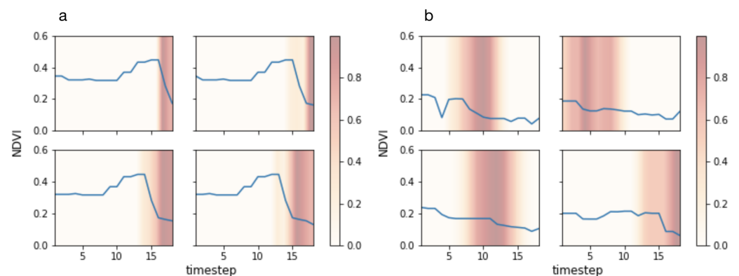
Figure 4. Saliency of temporal regions in time series for pixels in which land cover change is predicted to have occurred, determined using Grad-CAM++. Higher saliency scores indicates that the region is more influential in determining that land cover change has occurred. Blue lines show NDVI, though saliency is calculated using all input features. In a) a single pixel is shown at four points in time, with each subsequent panel shifted forward 1 step (10 days). In b) time series' from four spatially and temporal independent pixels are shown.
