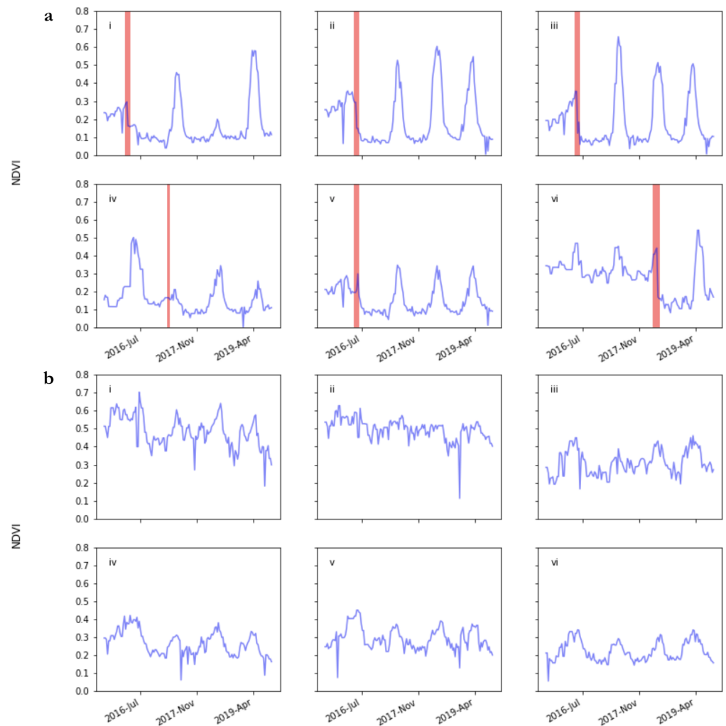
Figure 3. Observed NDVI time series for the full period covered by training and validation data for randomly selected pixels from across the study region. Vegetation in all time series' begins as natural Renosterveld. In panel a, a land cover change event occurs in the period highlighted in red, and thereafter the land cover is non-natural. In b, vegetation remains natural for the entire time series
