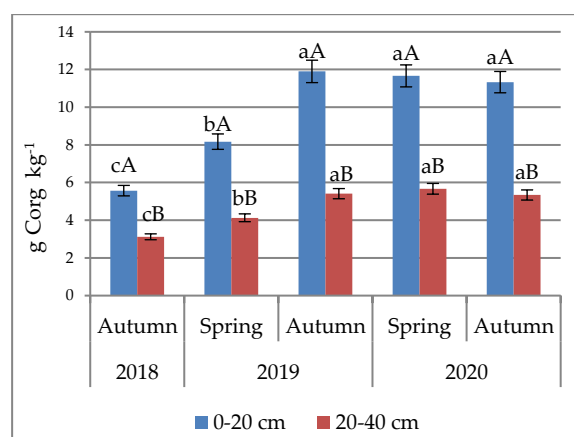
Figure 1. Content of organic carbon (Corg) in the studied soil. Different lower-case letters indicate significant differences among the dates (year) of soil sampling. Different upper-case letters indicate significant differences among levels of sampling.
