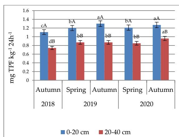
Figure 5. Activity of dehydrogenases (DEH) in the studied soil. Different lower-case letters indicate significant differences among the dates (year) of soil sampling. Different upper-case letters indicate significant differences among the levels of sampling.
