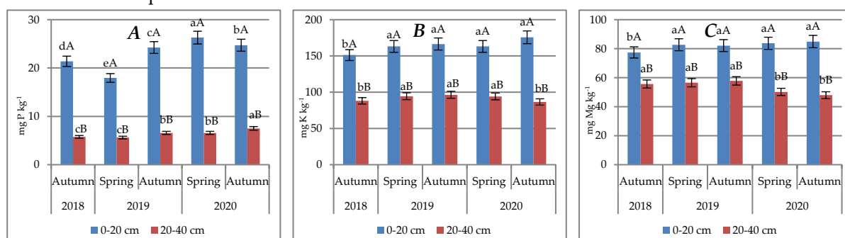
Figure 2. A, B, and C. Contents of available P (A), K (B), and Mg (C) in the studied soil. Different lower-case letters indicate significant differences among the dates (year) of soil sampling. Different upper-case letters indicate significant differences among the levels of sampling. Bars represent standard deviation.
