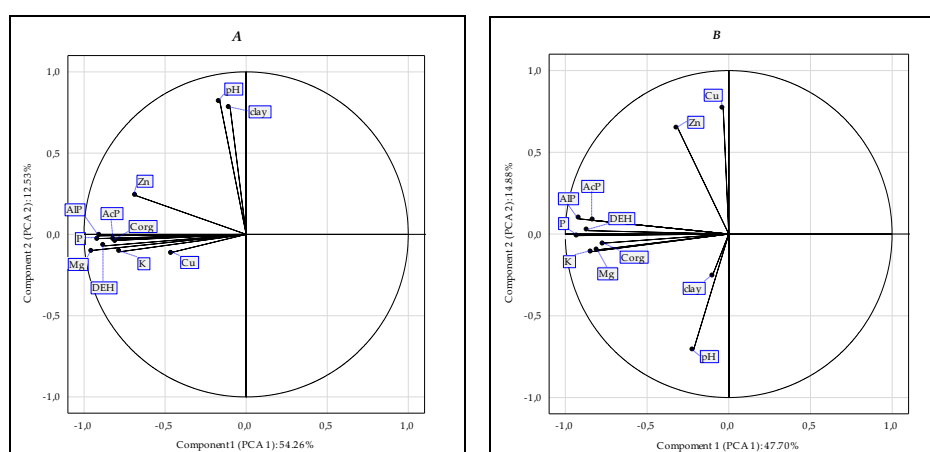
Figure 7. A and B. Configuration of variables in the system of the first two axes PC1 and PC2 of principal components in the soil after application destillery stillage A (2019 year) and B (2020 year).
