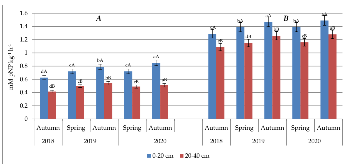
Figure 4. Activity of alkaline (AIP) and acid (AcP) phosphatases in the studied soil. Different lower-case letters indicate significant differences among the dates (year) of soil sampling. Different upper-case letters indicate significant differences among the levels of sampling.
