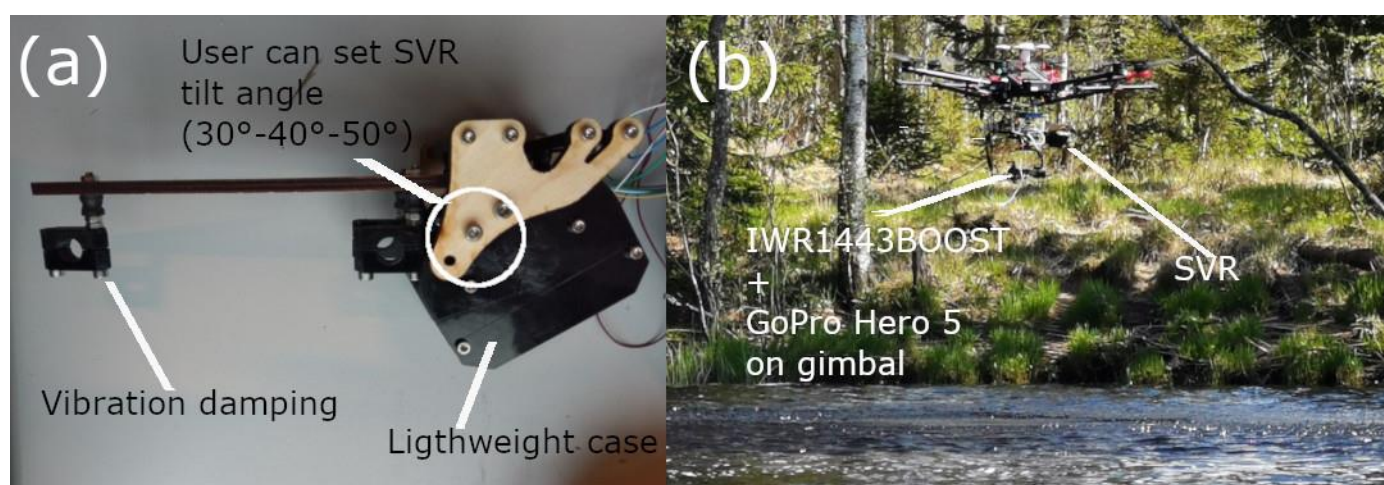
Figure 1. Pictures of UAS payload. (a) SVR adaption for being used as drone payload (b) UAS flight with SVR Doppler radar, IWR1443BOOST radar and GoPro Hero 5 RGB camera.
