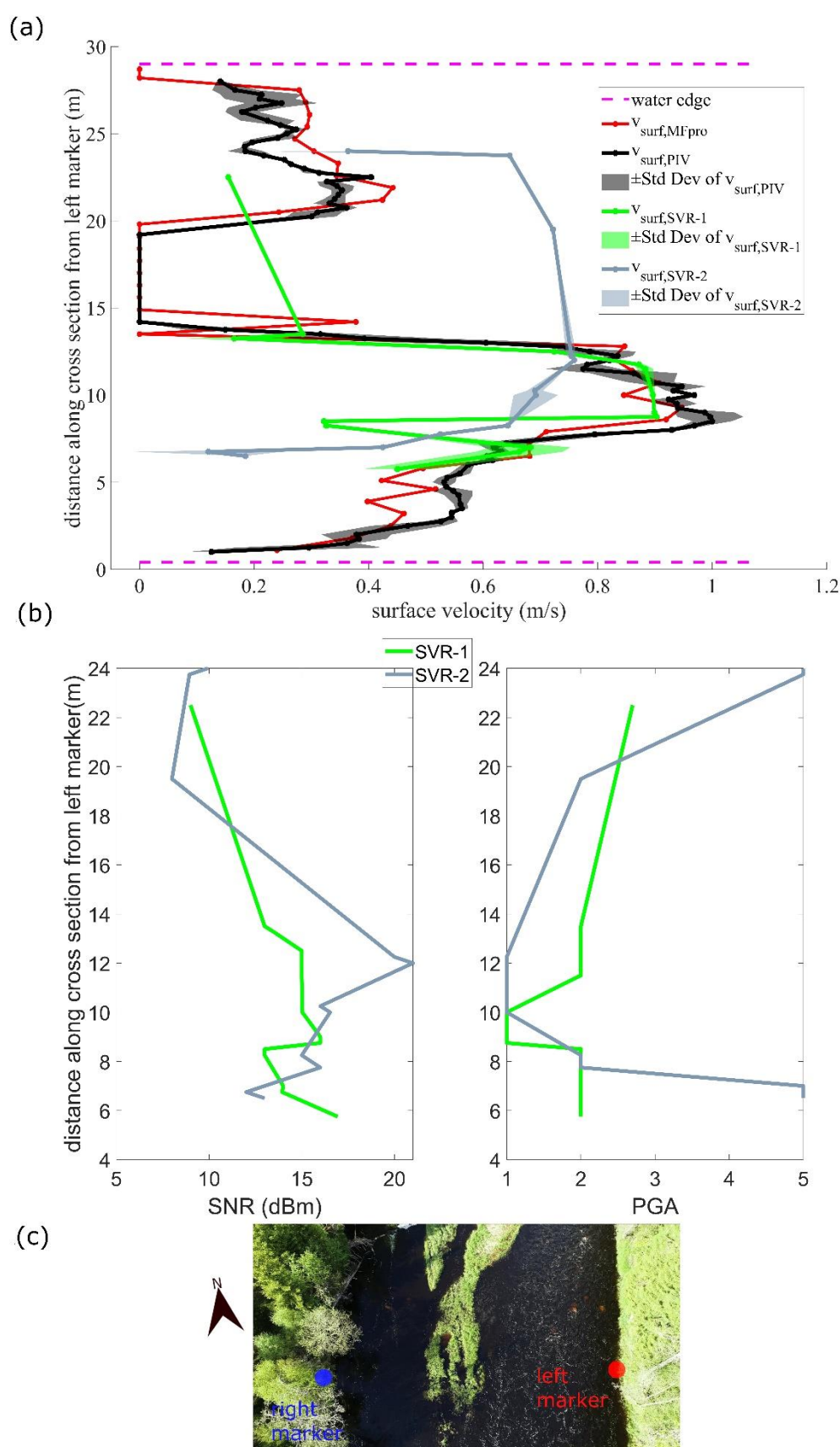
Figure 7, Kilan XS. (a) surface velocity comparing: MFpro measurements of surface velocity ( v_{\text{surf,MFpro}} ), UAS-borne PIV measurements ( v_{\text{surf,PIV}} ) and two UAS-borne SVR ( v_{\text{surf,SVR-1}} , v_{\text{surf,SVR-2}} , all
