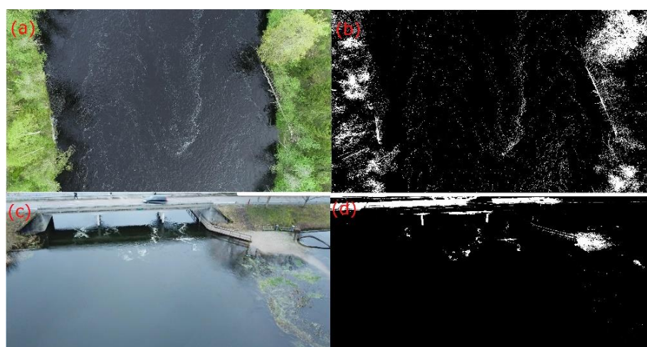
Figure 3. A mask was applied to the RGB video frames (left panel) to obtain a binary image (right panels): white color is assigned to seeding, whilst a black color is assigned to water surface (with a few outlier). (a) and (b) are in case of natural seeding (mainly foam), whilst (c) and (d) are in case of artificial seeding (woodchips).
