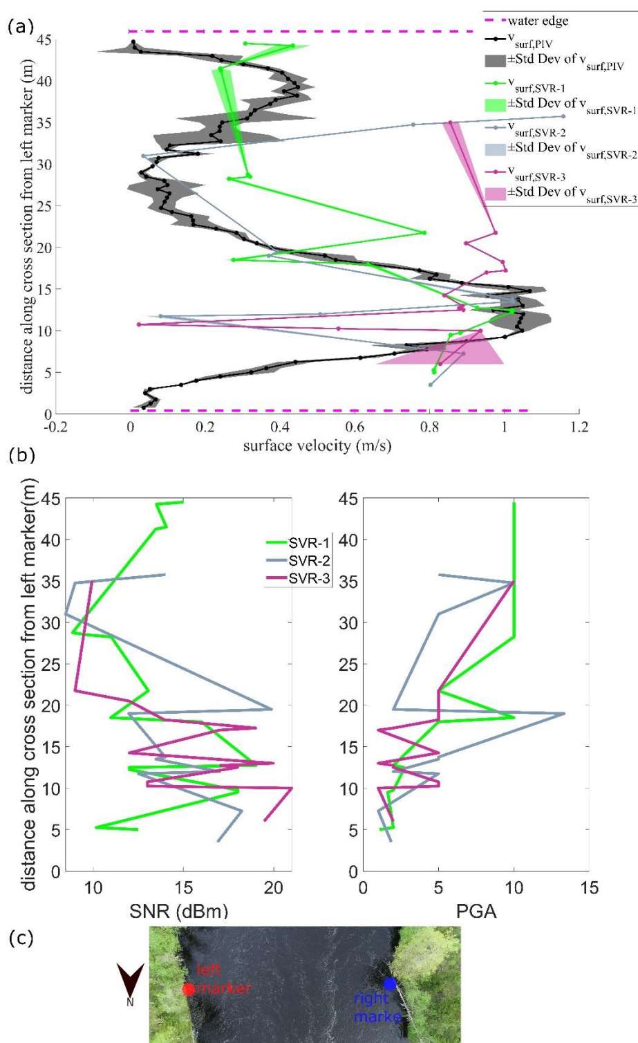
Figure 6, Ätran XS. (a) surface velocity comparing: UAS-borne PIV measurements ( v_{surf,PIV} ) and three UAS-borne SVR ( v_{surf,SVR-1} , v_{surf,SVR-2} and v_{surf,SVR-3} , all of which pointing upstream) surveys. SVR and PIV are represented with shaded regions to present standard deviation ( \pm Std Dev). (b) Comparison of two quality indicators (SNR and PGA) for the SVR surveys. (c) UAS-borne video frame of the XS (North arrow is also shown).
