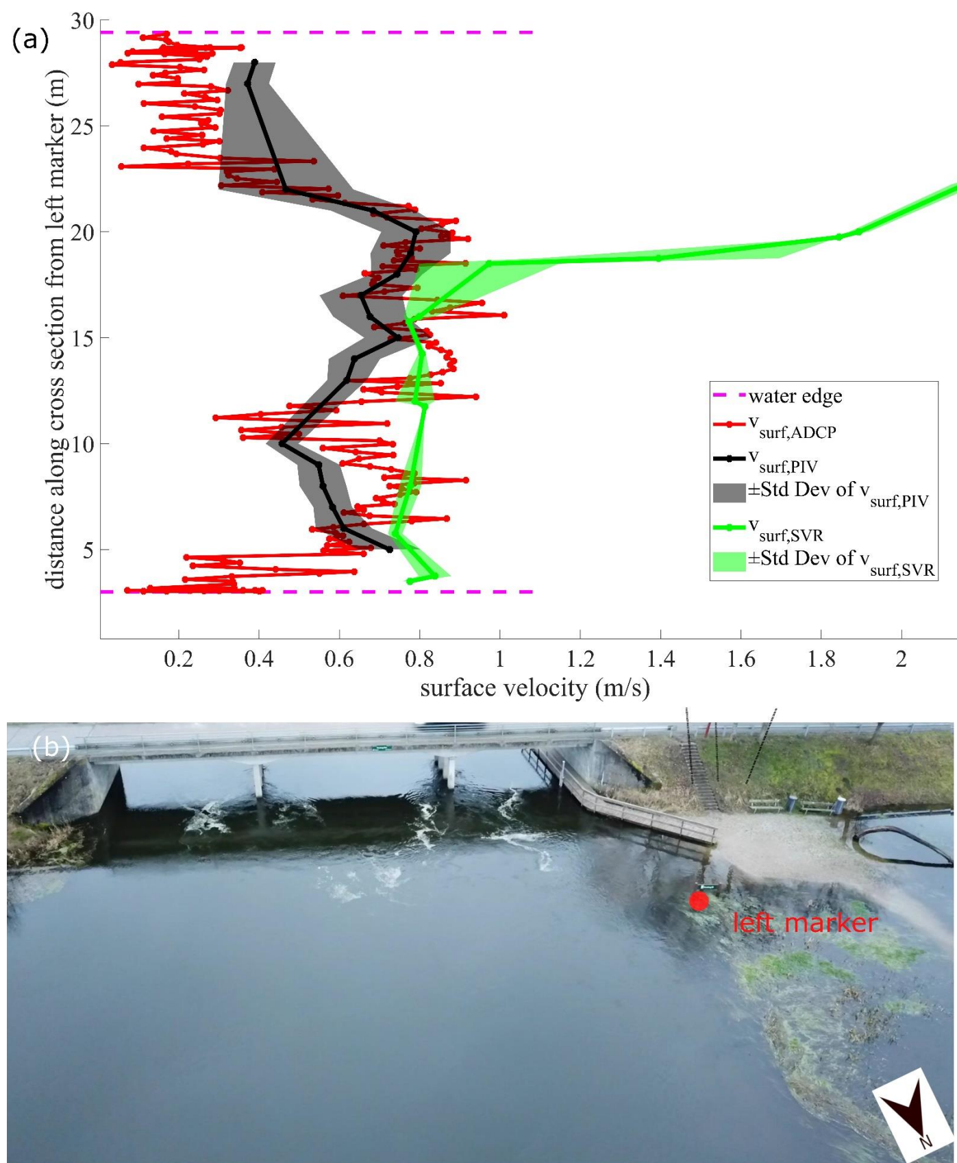
Figure 4, Gudensøvostrupvej XS. (a) surface velocity plot comparing: ADCP measurements of surface velocity ( v_{surf,ADCP} ), UAS-borne PIV ( v_{surf,PIV} ) and UAS-borne SVR ( v_{surf,SVR} ). SVR and PIV are represented with shaded grey (PIV) and shaded green (SVR) to present standard deviation ( \pm Std
