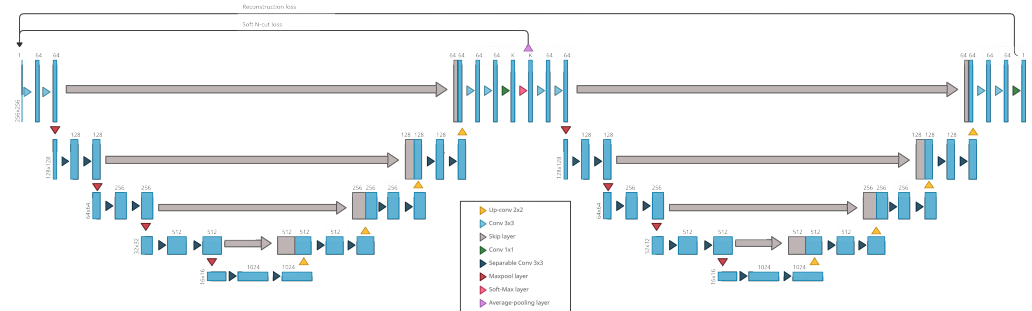
Figure 2. Our W-net architecture for ARMD lesions segmentation
