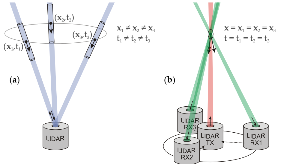
Figure 2. (a) A conventional monostatic lidar uses a single combined transmitter and receiver, resulting in a large measurement volume which needs to be multiplexed spatially and temporally by sequentially tilting the beam and sampling the wind speed. (b) The PTB bistatic lidar uses three separate receivers (RX1, RX2, RX3) around a central transmitter (TX), facilitating the simultaneous measurement of the three wind velocity components with high spatial and temporal resolution.
