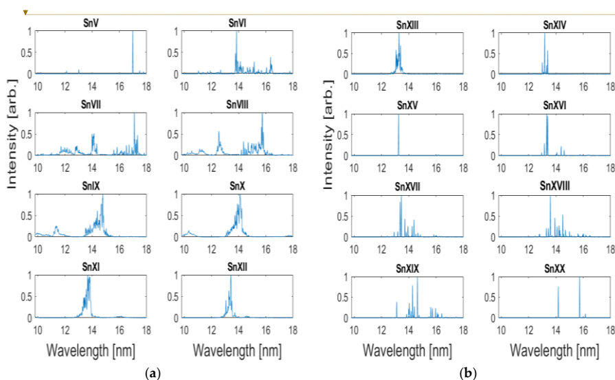
Figure 3: Theoretical spectra calculated with the Cowan suite of codes for Sn V - Sn XX ions, weighted transition probabilities are convolved with a Gaussian of width 0.01 nm and normalized in the 9.8 - 18 nm region. (See text.)
