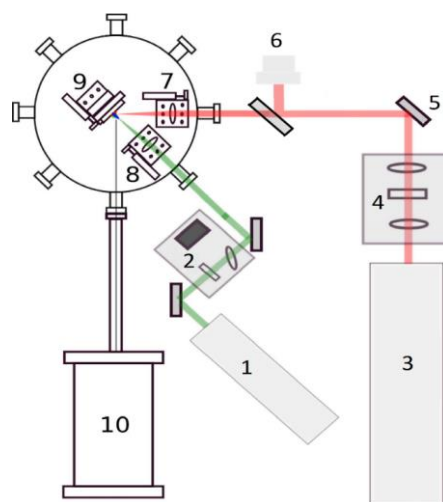
Figure 1: Experimental layout; 1 : Nd:YAG laser, 2 : Nd:YAG energy selector, 3 : CO 2 laser, 4 : plasma shutter, 5 : steering mirror, 6 : pulse profiler, 7 : CO 2 focusing lens, 8 : Nd:YAG focusing lens, 9 : x, y, z target motion, 10 : spectrometer.
