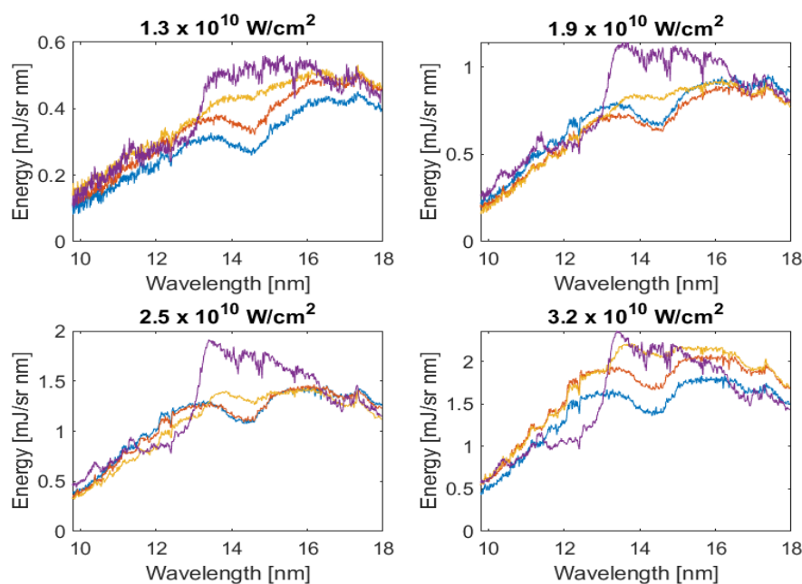
Figure 7: Spectra recorded for a fixed spot radius of 300 \mu\text{m} ; the laser energies were 185 mJ, 270 mJ, 350mJ, 450 mJ; blue: Pb, red: PbSn946, yellow: PbSn6535 and purple: Sn.
