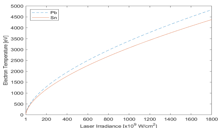
Figure 2: Ion stage populations for Pb (a) and Sn (b) plasmas for electron temperatures of 10 eV – 100 eV. The bottom graph (c) shows electron temperature as a function of input laser irradiance.
