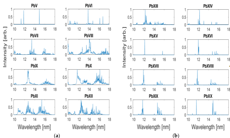
Figure 5: Theoretical spectra calculated with the Cowan code for Pb V - Pb XX ions, the weighted transition probabilities are convolved with a Gaussian of width 0.01 nm and normalized in the 9.8 - 18 nm region. (See text.)
