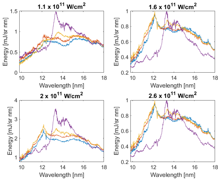
Figure 9: Spectra recorded for a fixed spot radius of 100 \mu m, the laser energies were 185 mJ, 270 mJ, 350mJ, 450 mJ; blue: Pb, red: PbSn946, yellow: PbSn6535 and purple: Sn.
