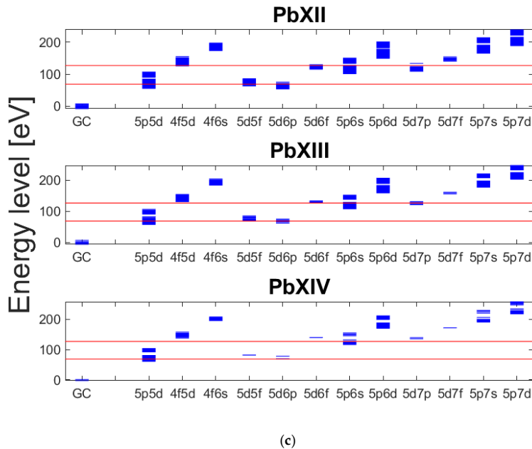
Figure 14: Relevant energy levels of excited configurations in Pb VI to Pb XIV taken from the Cowan code calculations; GC represents the ground configuration, 5d^9 to 5d^1 . The red lines indicate the approximate region of interest. (See text.)
