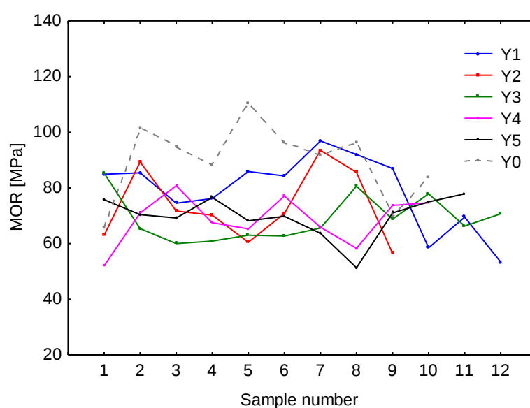
Figure 5. The radial variability for static bending resistance (MOR) of spruce wood depending on the period of time since the tree's decay.
