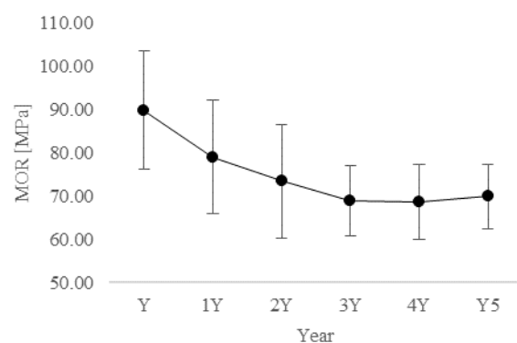
Figure 3. Resilience to static bending (MOR) of spruce wood in reference to the time since the tree's decay.
