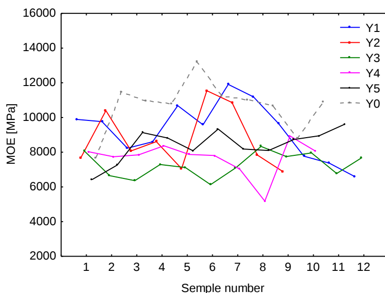
Figure 6. The radial variability of modulus of elasticity (MOE) of spruce wood depending on the period of time since the tree's decay.
