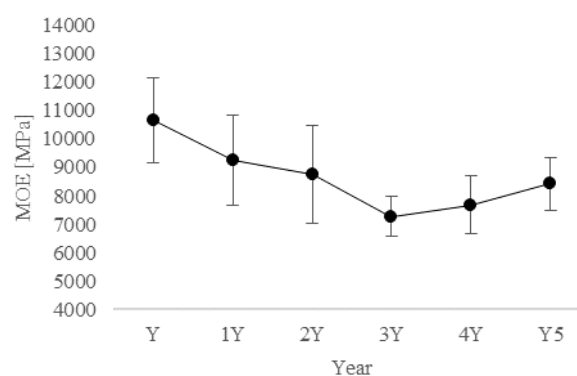
Figure 4. Modulus of elasticity (MOE) of spruce wood in reference to the time since the tree's decay.
